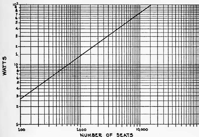
FIG. 1. Variation of required electric output with number of seats.
